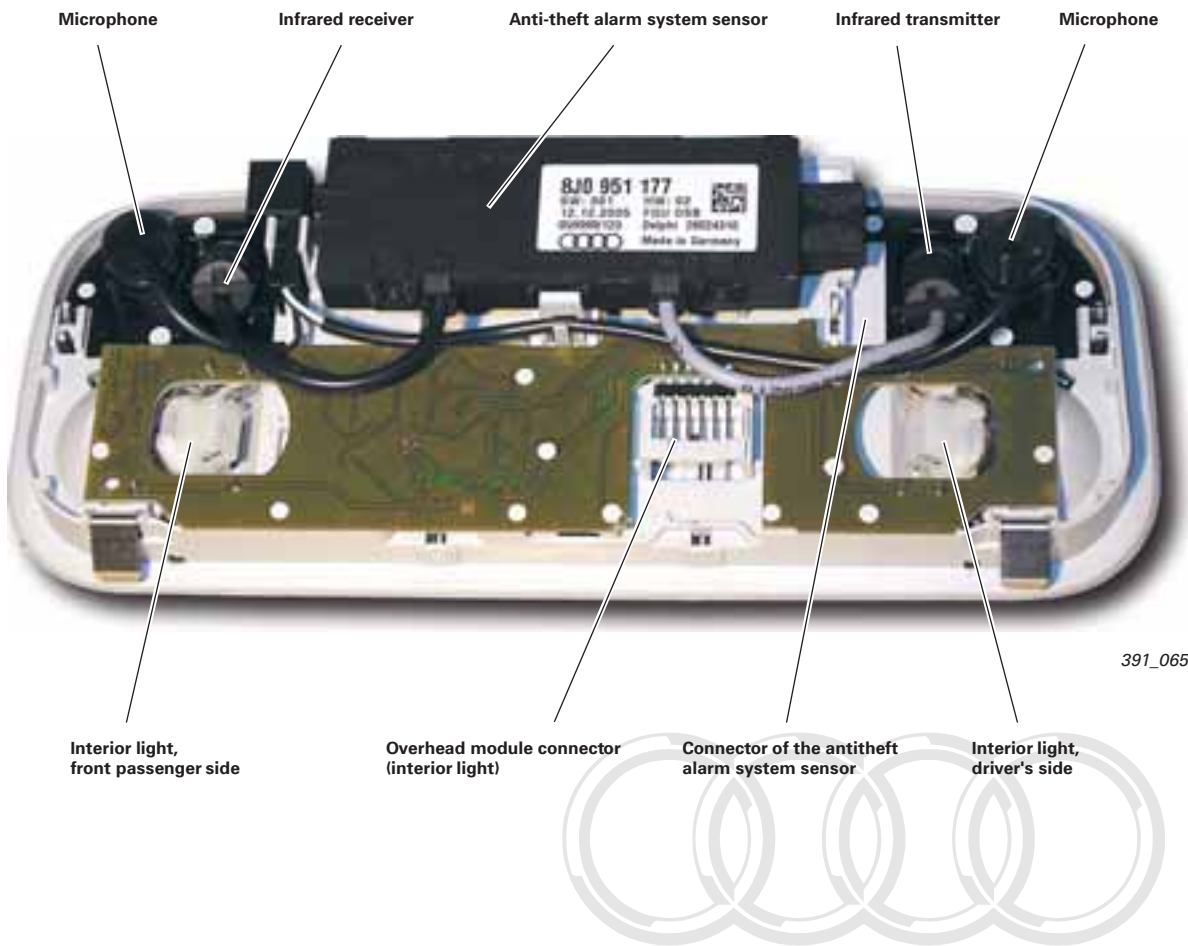
Overhead module with anti-theft alarm sensor G578
